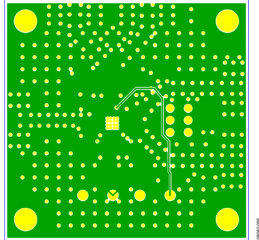
Figure 52. Evaluation Board Power Plane, Internal Layer 2
