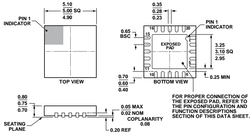
COMPLIANT TO JEDEC STANDARDS MO-220-WHHC. Figure 54. 20-Lead Lead Frame Chip Scale Package [LFCSP_WQ] 5 mm × 5 mm Body, Very Very Thin Quad (CP-20-9) Dimensions shown in millimeters
